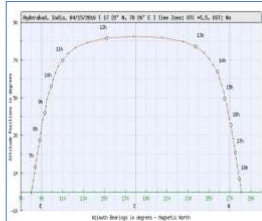
Figure 6 sun position graph
