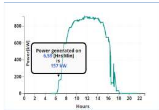
Figure 8 output power of dual axis solar tracker
