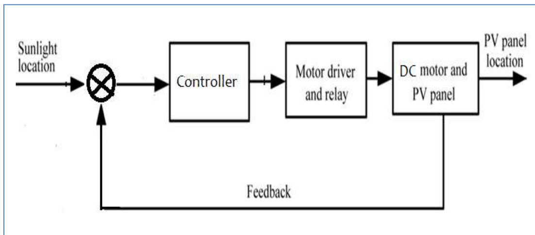
Figure 1 Block diagram of dual axis solar tracking system
