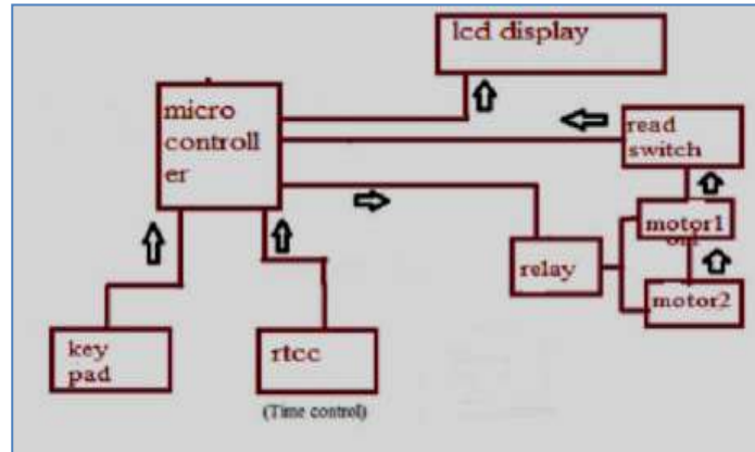
Figure 2 Block diagram of solar tracker control
