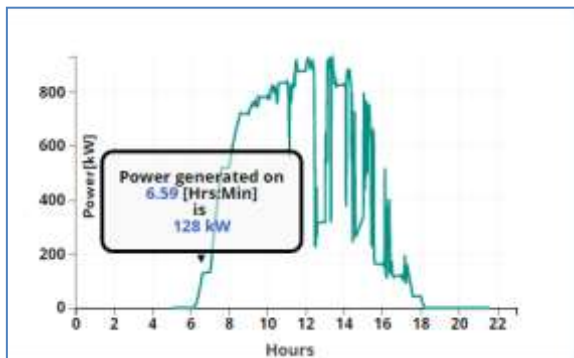
Figure 7 output power of single axis solar tracker
